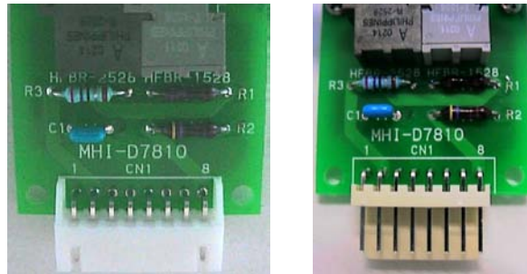
OCB: old connector (left) and new connector (right)
